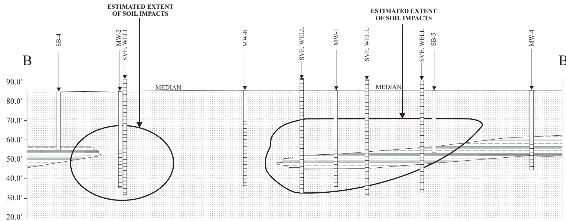
CROSS SECTION B - B'
